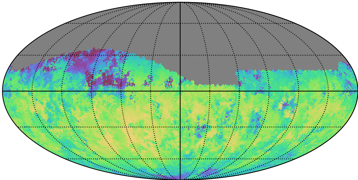
baseline_v3.3_10yrs Yr 1 z band: Median skyBrightness
