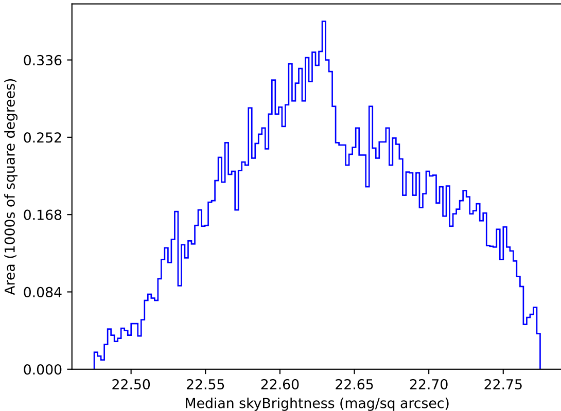
baseline_v3.3_10yrs Yr 1 u band: Median skyBrightness
