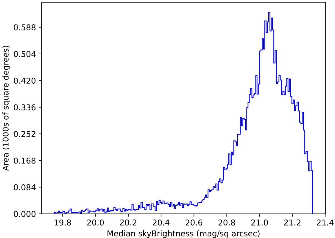
baseline_v3.3_10yrs Yr 1 r band: Median skyBrightness
