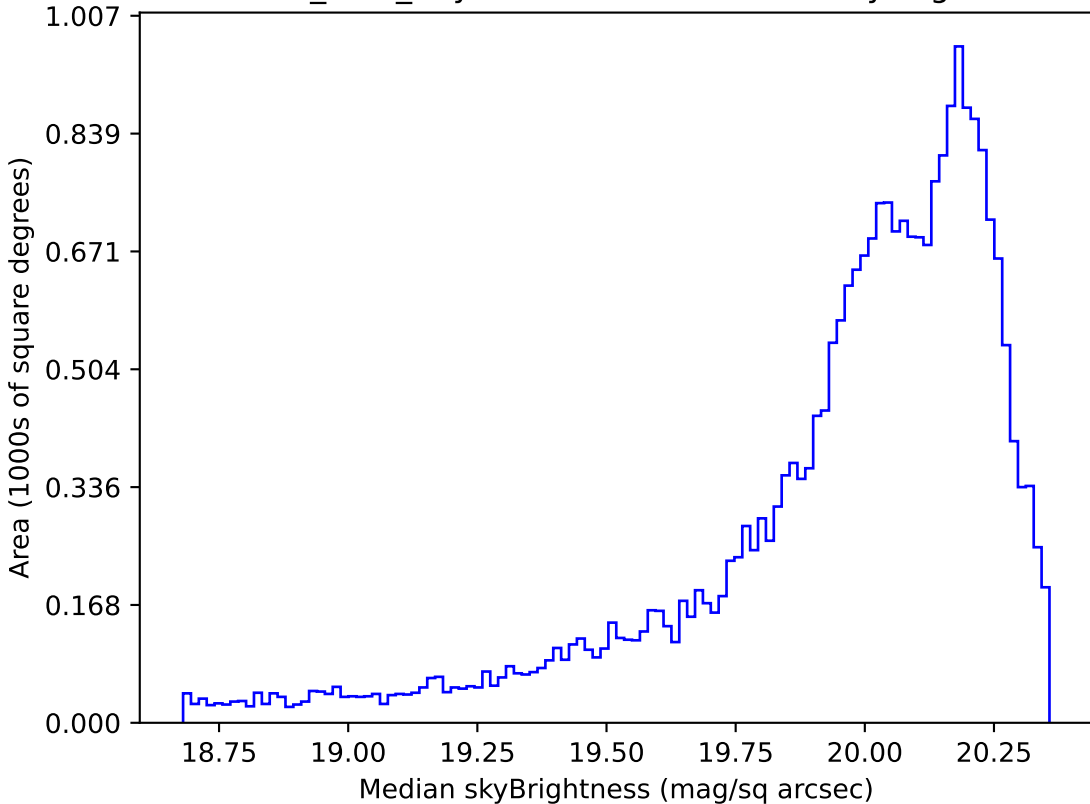
baseline_v3.3_10yrs Yr 1 i band: Median skyBrightness
