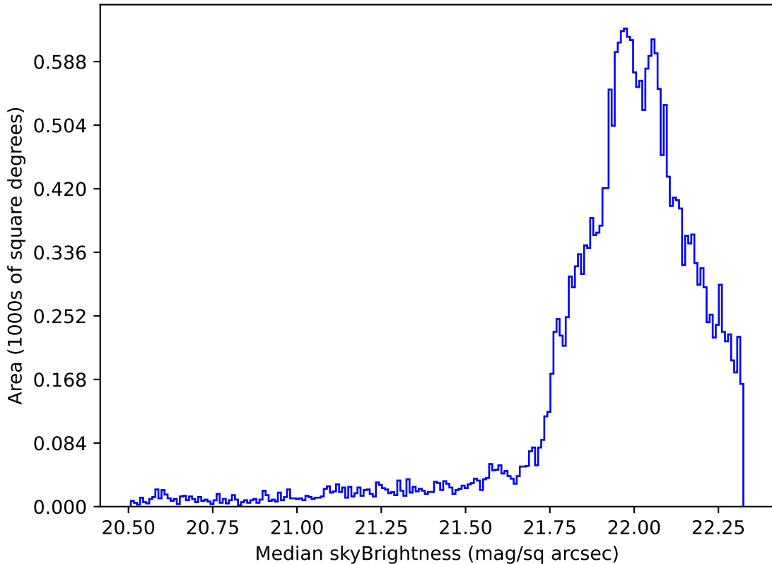
baseline_v3.3_10yrs Yr 1 g band: Median skyBrightness
