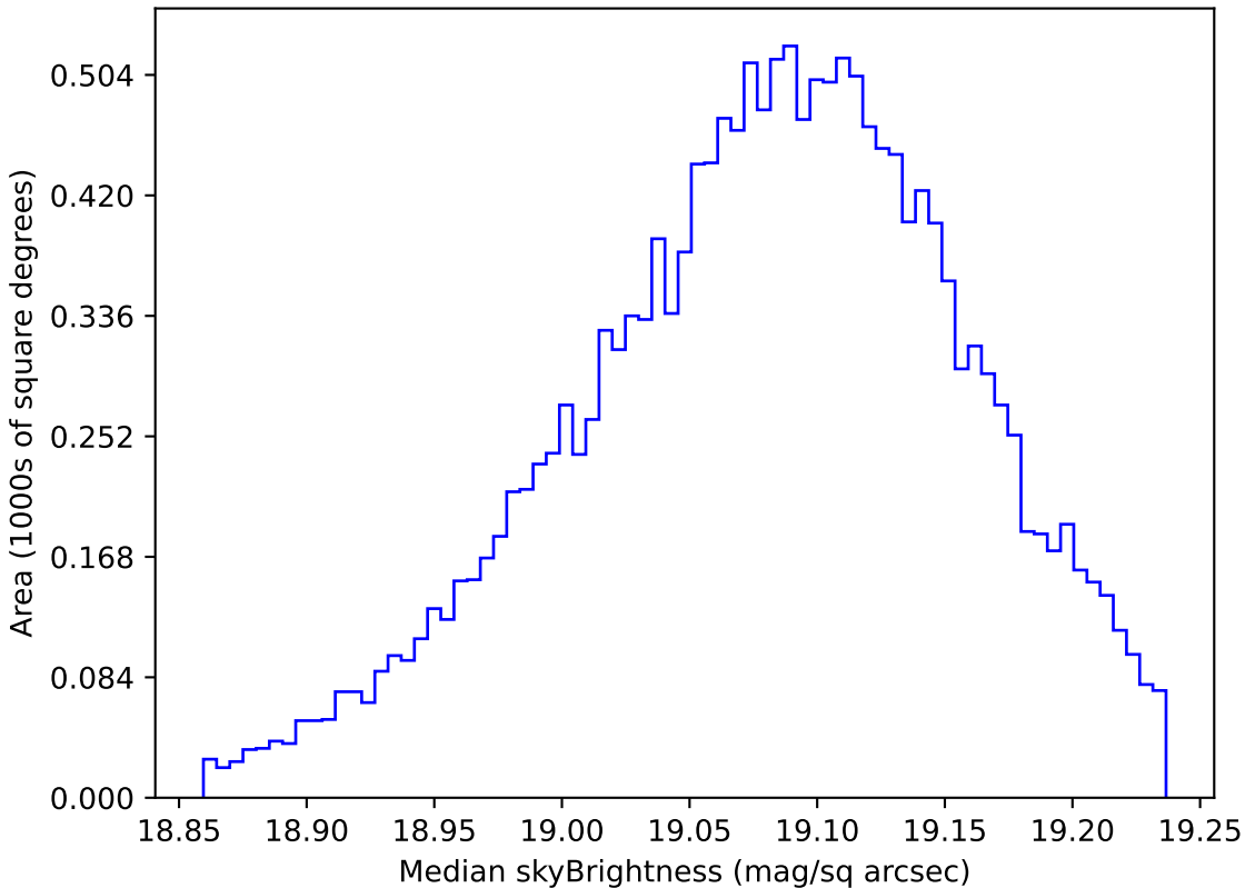
baseline_v3.3_10yrs WFD z band: Median skyBrightness
