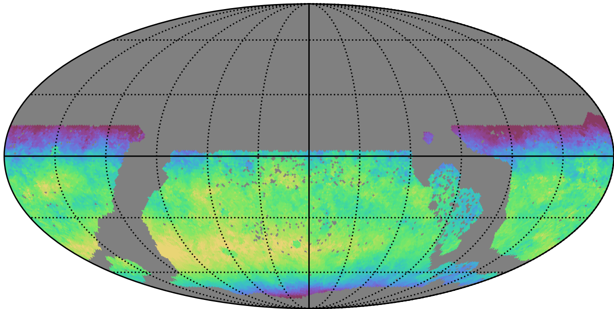
baseline_v3.3_10yrs WFD y band: Median skyBrightness
