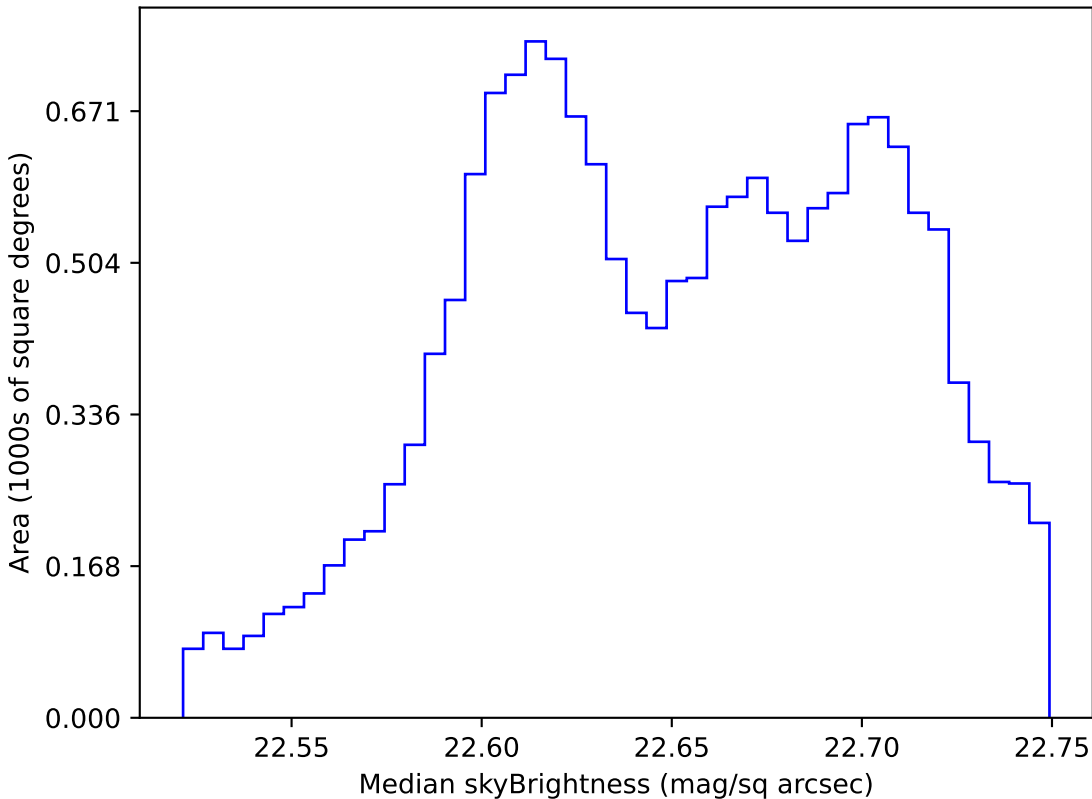
baseline_v3.3_10yrs WFD u band: Median skyBrightness
