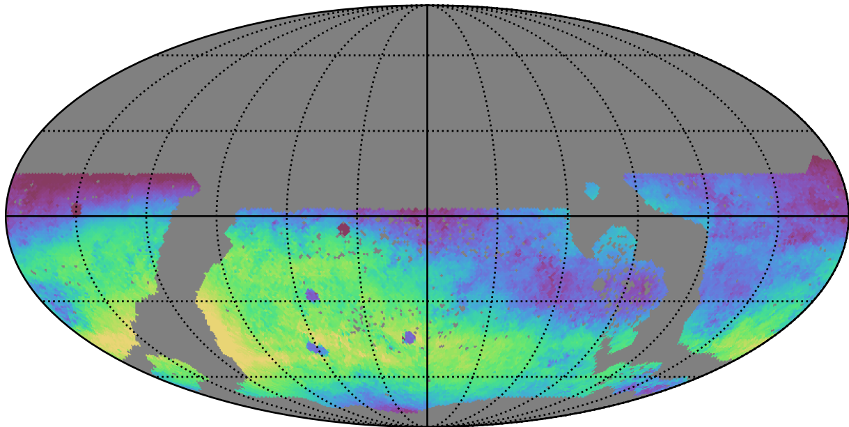
baseline_v3.3_10yrs WFD r band: Median skyBrightness
