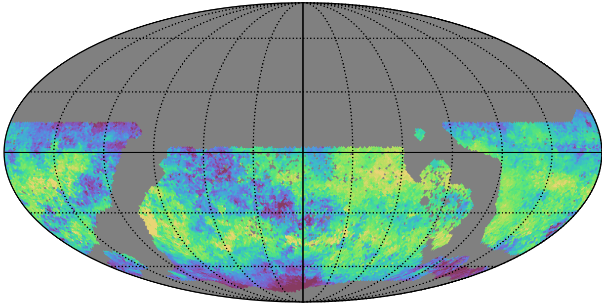
baseline_v3.3_10yrs WFD i band: Median skyBrightness
