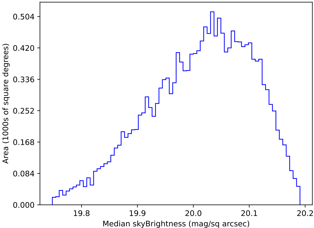
baseline_v3.3_10yrs WFD i band: Median skyBrightness
