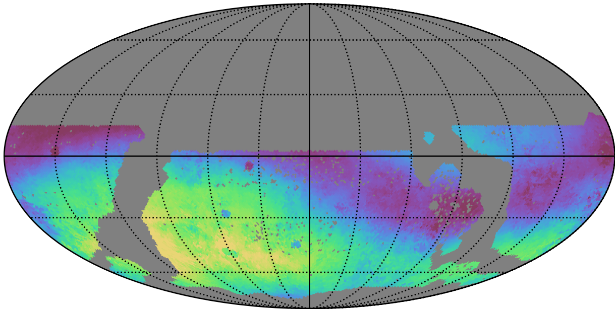
baseline_v3.3_10yrs WFD g band: Median skyBrightness
