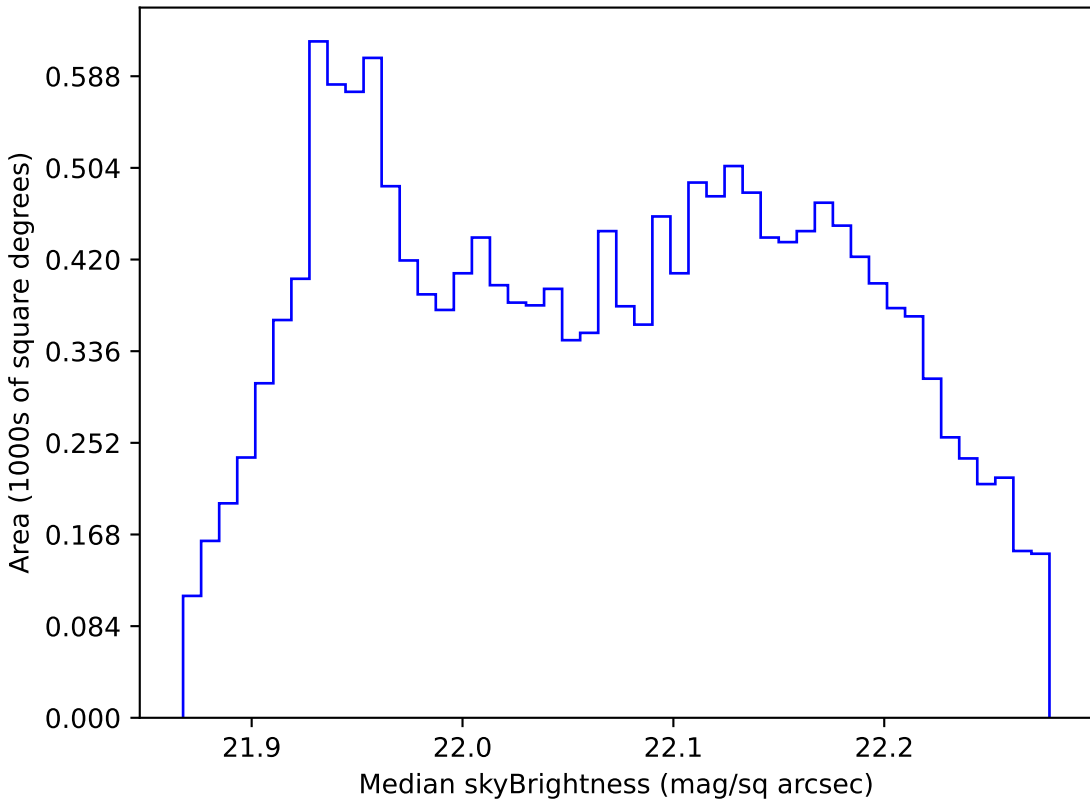
baseline_v3.3_10yrs WFD g band: Median skyBrightness
