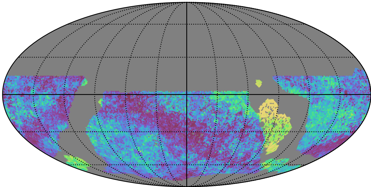
baseline_v3.3_10yrs WFD all bands: Median skyBrightness
