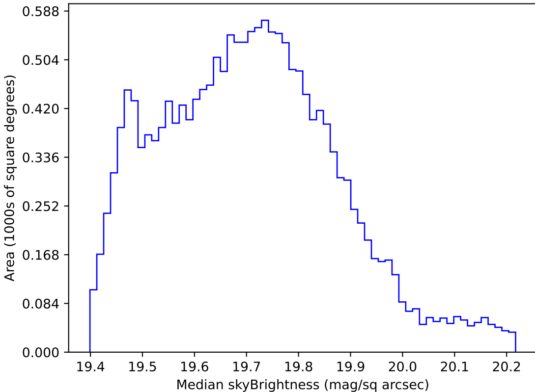
baseline_v3.3_10yrs WFD all bands: Median skyBrightness
