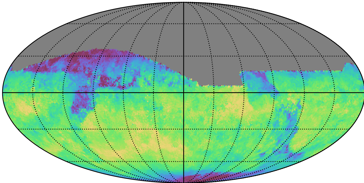
baseline_v3.3_10yrs All sky z band: Median skyBrightness
