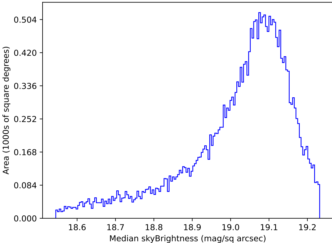
baseline_v3.3_10yrs All sky z band: Median skyBrightness
