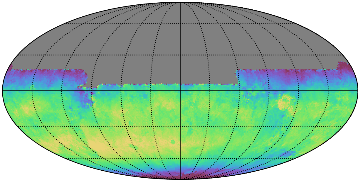
baseline_v3.3_10yrs All sky y band: Median skyBrightness
