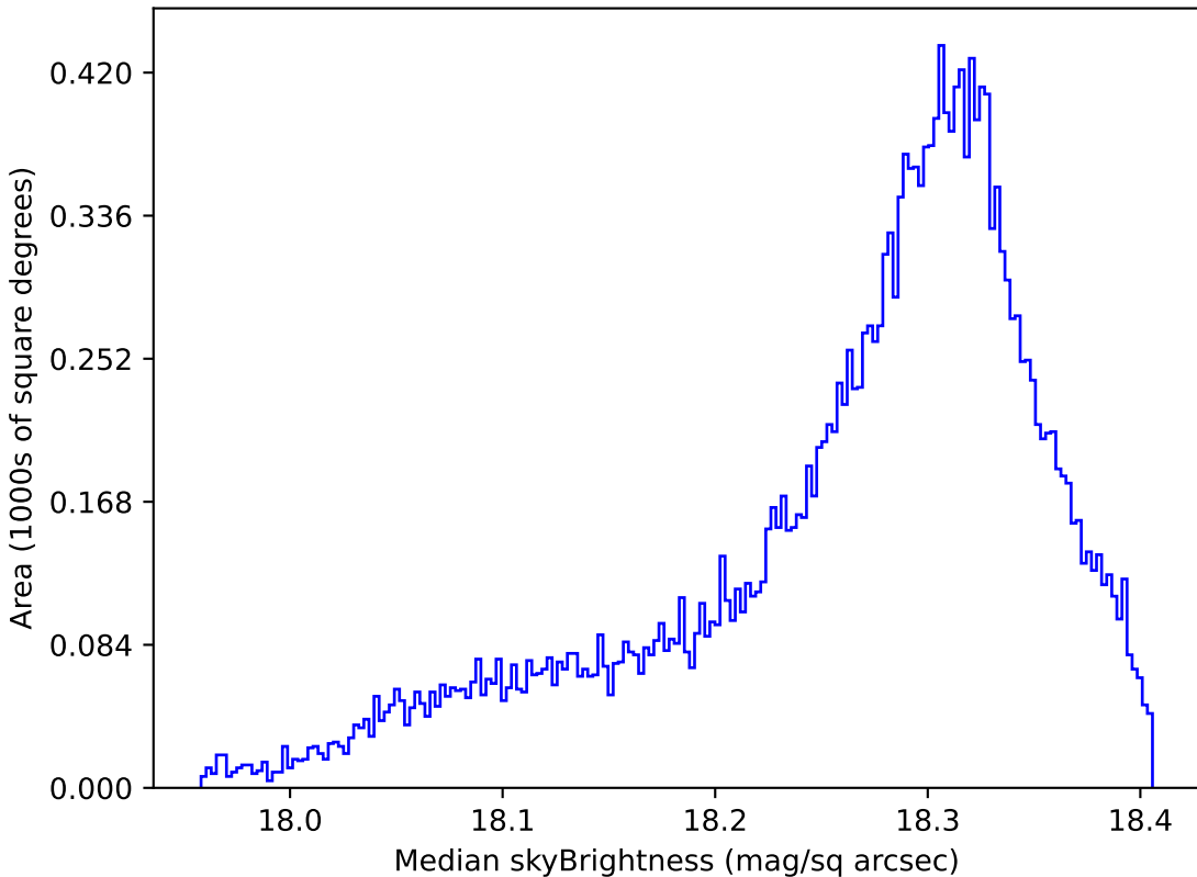
baseline_v3.3_10yrs All sky y band: Median skyBrightness
