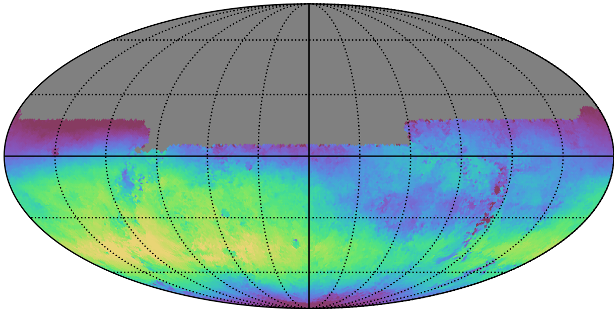
baseline_v3.3_10yrs All sky u band: Median skyBrightness
