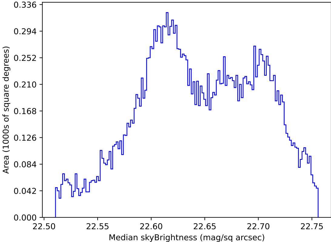
baseline_v3.3_10yrs All sky u band: Median skyBrightness
