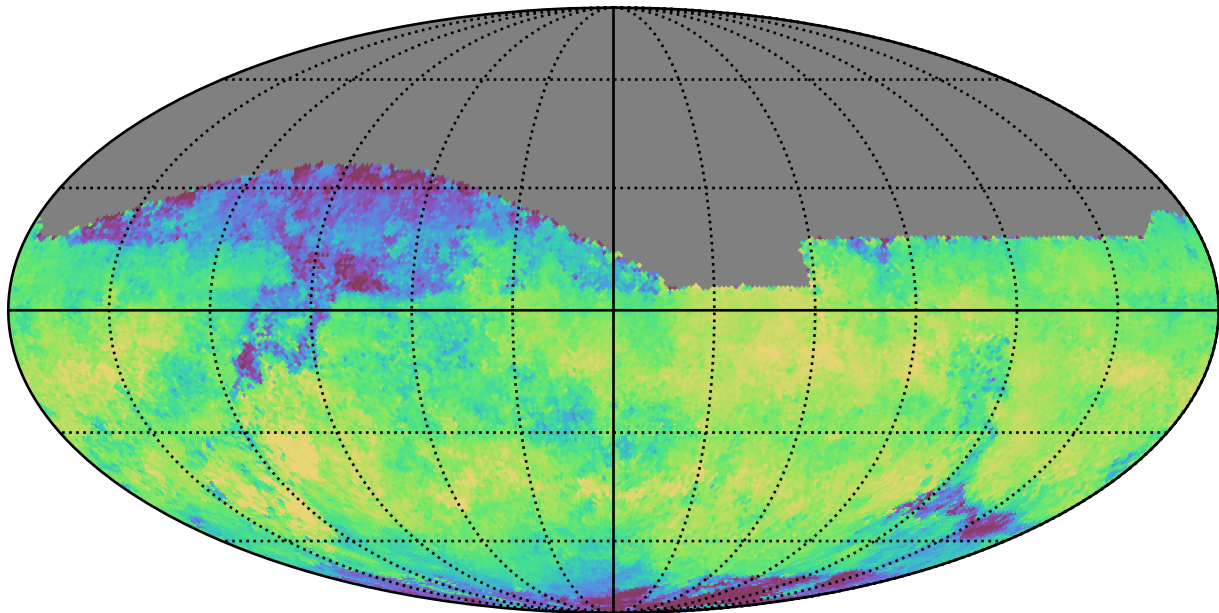
baseline_v3.3_10yrs All sky i band: Median skyBrightness
