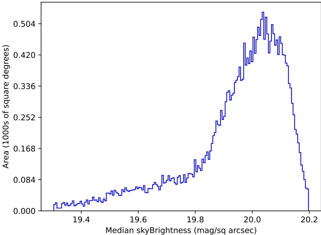
baseline_v3.3_10yrs All sky i band: Median skyBrightness
