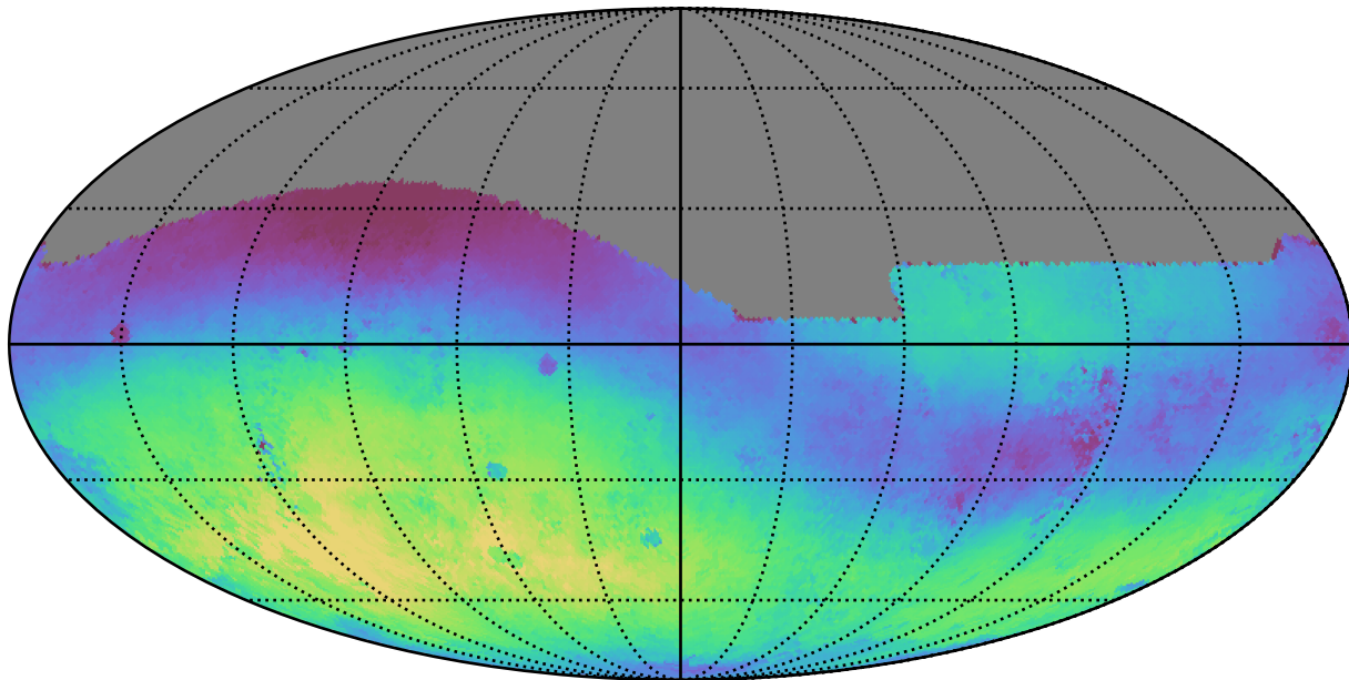
baseline_v3.3_10yrs All sky g band: Median skyBrightness
