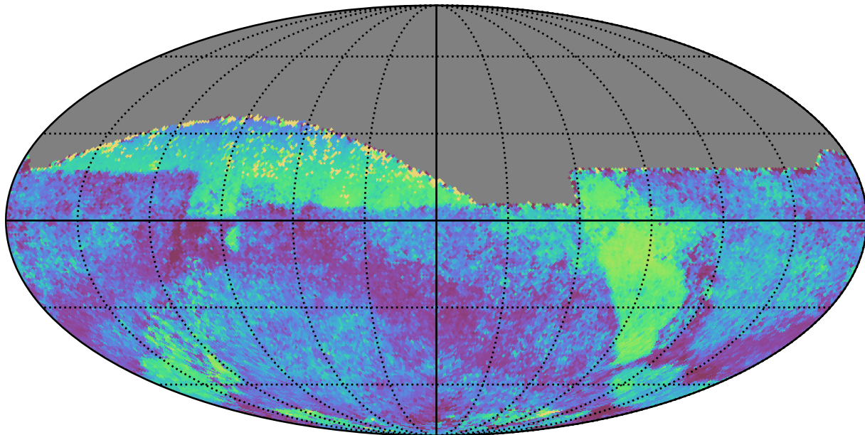
baseline_v3.3_10yrs All sky all bands: Median skyBrightness
