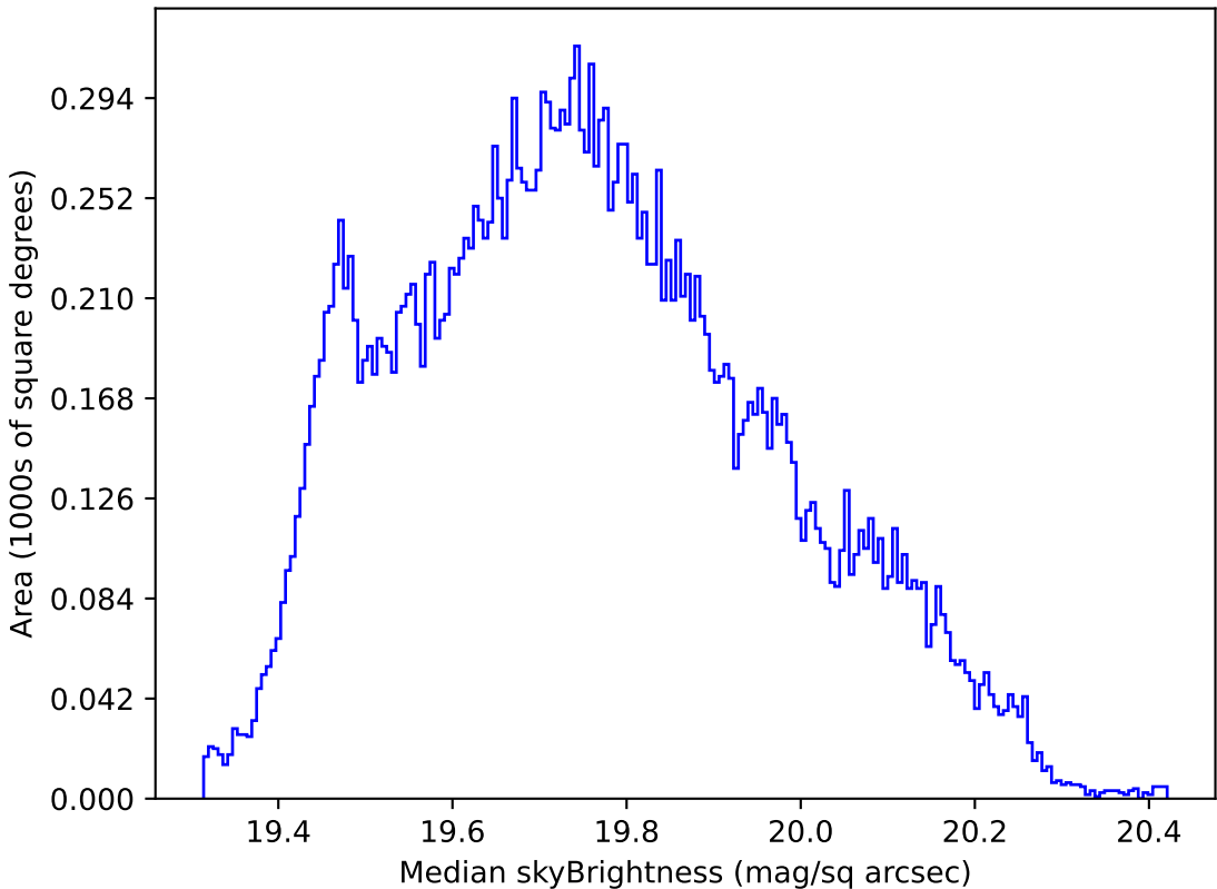
baseline_v3.3_10yrs All sky all bands: Median skyBrightness
