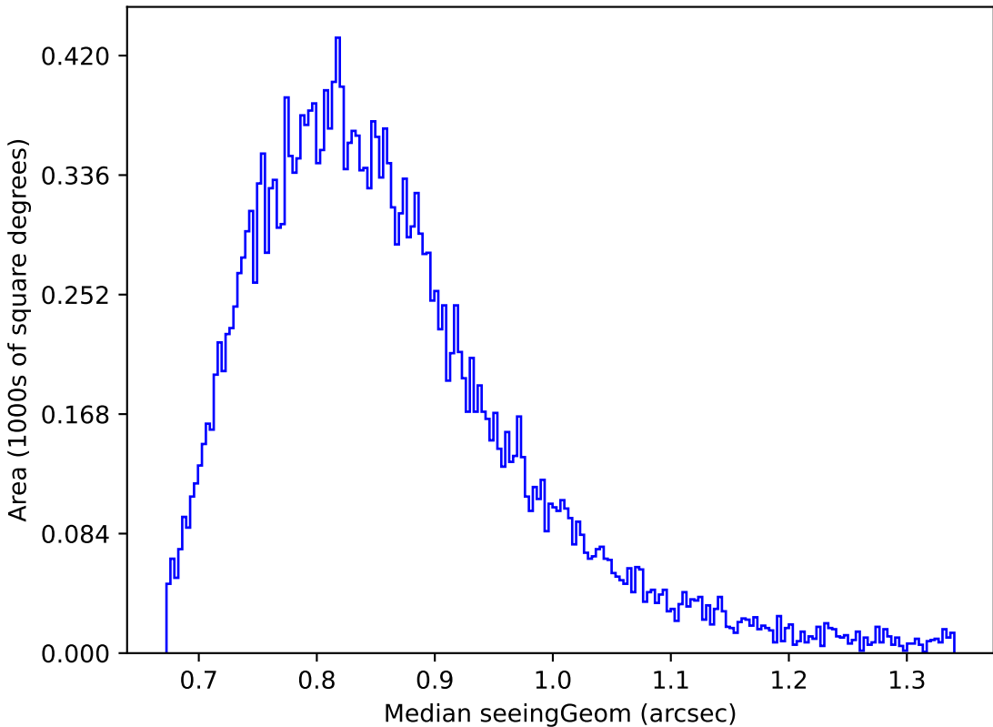
baseline_v3.3_10yrs Yr 1 z band: Median seeingGeom
