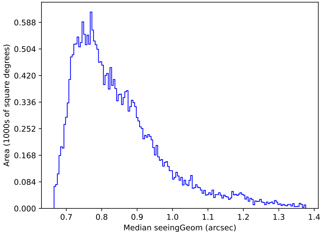
baseline_v3.3_10yrs Yr 1 r band: Median seeingGeom
