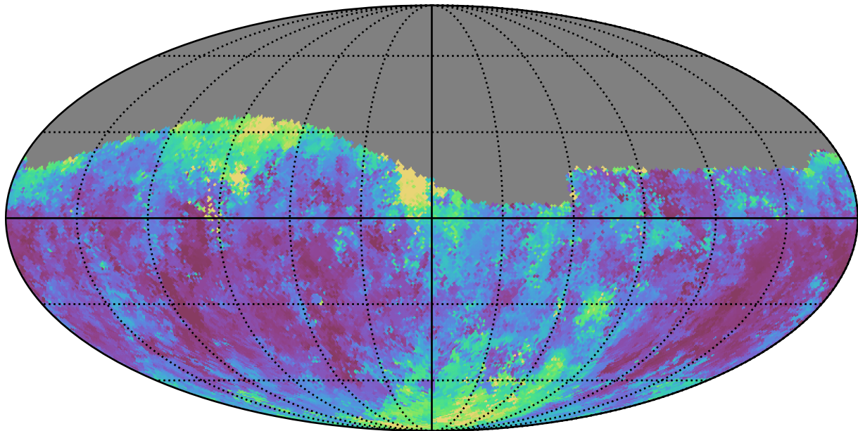
baseline_v3.3_10yrs Yr 1 g band: Median seeingGeom
