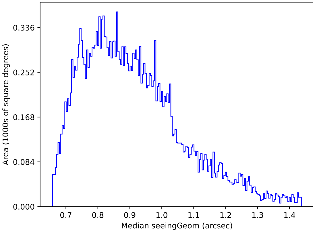
baseline_v3.3_10yrs Yr 1 g band: Median seeingGeom
