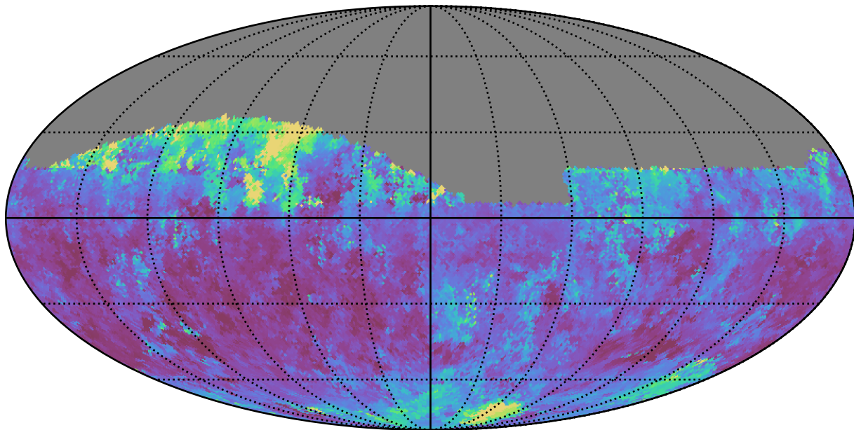
baseline_v3.3_10yrs Yr 1 z band: Median seeingEff
