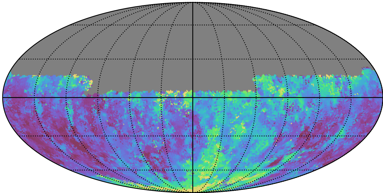
baseline_v3.3_10yrs Yr 1 u band: Median seeingEff
