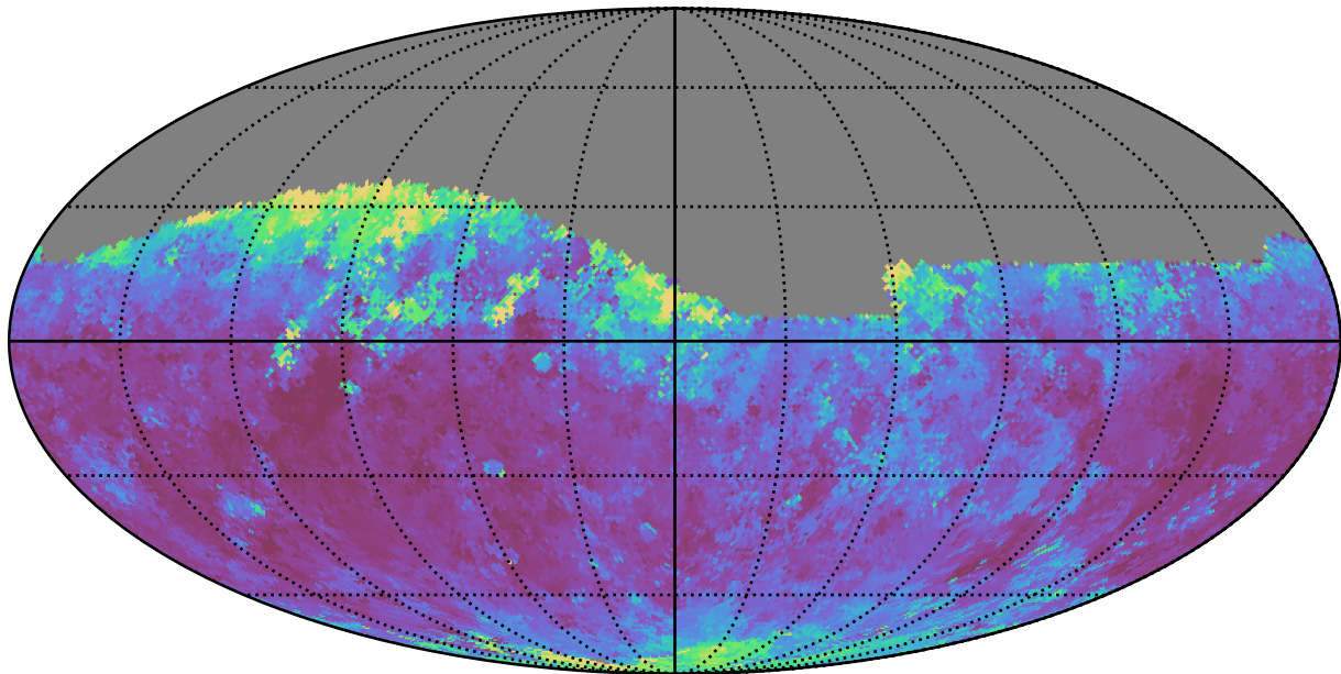
baseline_v3.3_10yrs Yr 1 r band: Median seeingEff
