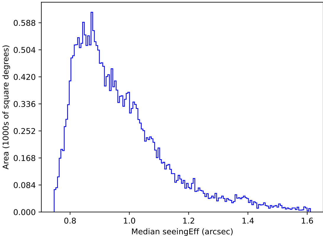
baseline_v3.3_10yrs Yr 1 r band: Median seeingEff
