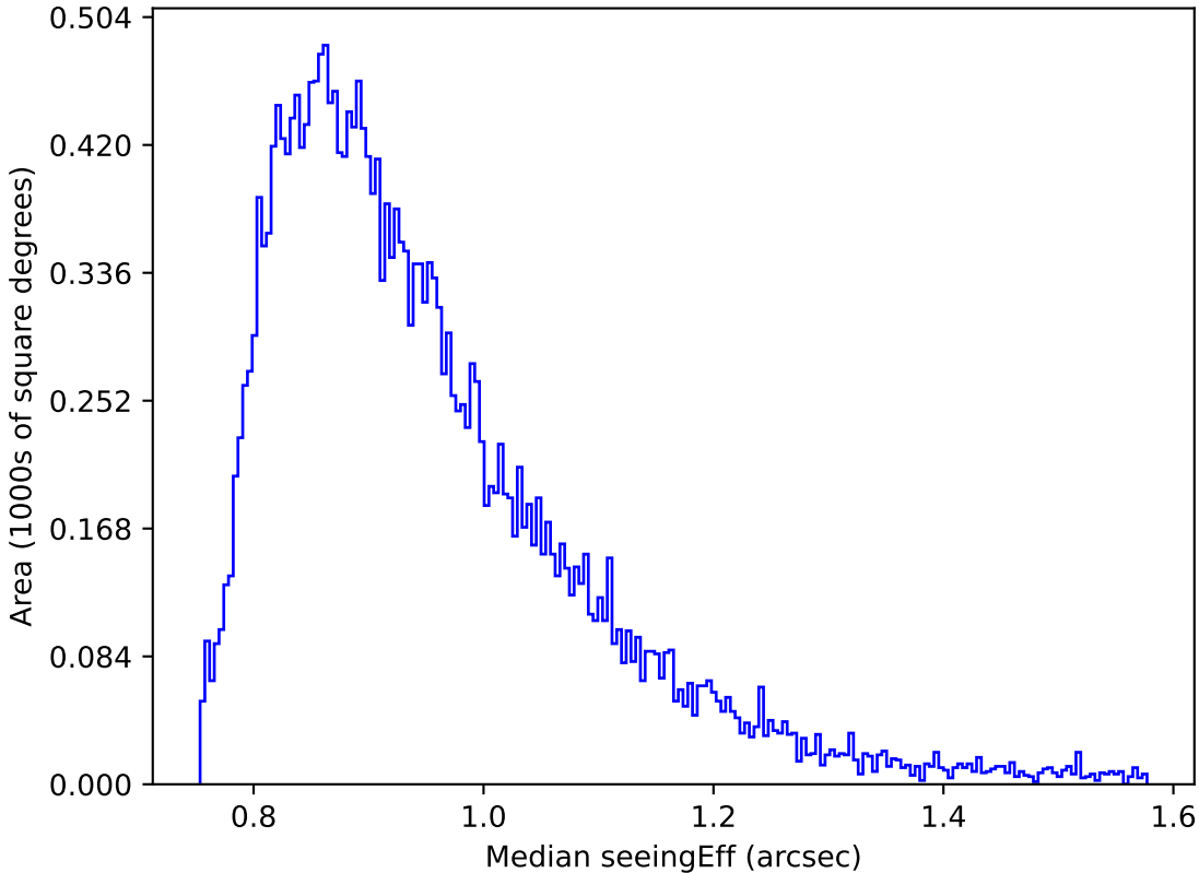
baseline_v3.3_10yrs Yr 1 i band: Median seeingEff
