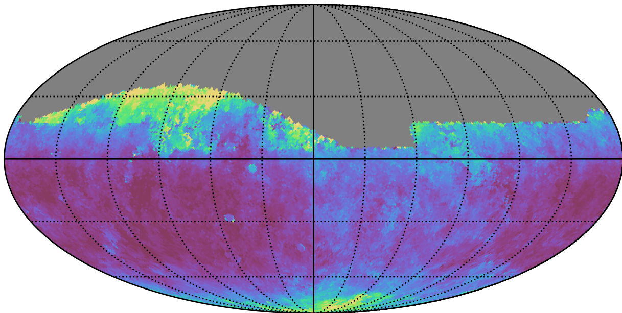
baseline_v3.3_10yrs Yr 1 all bands: Median seeingEff
