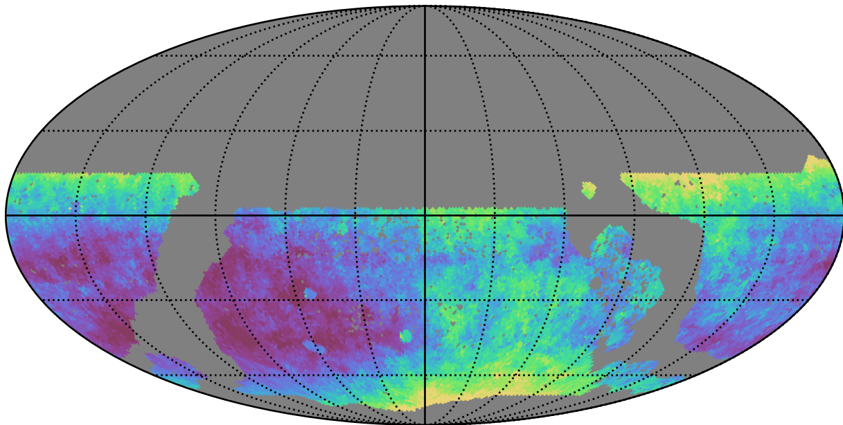
baseline_v3.3_10yrs WFD z band: Median seeingEff
