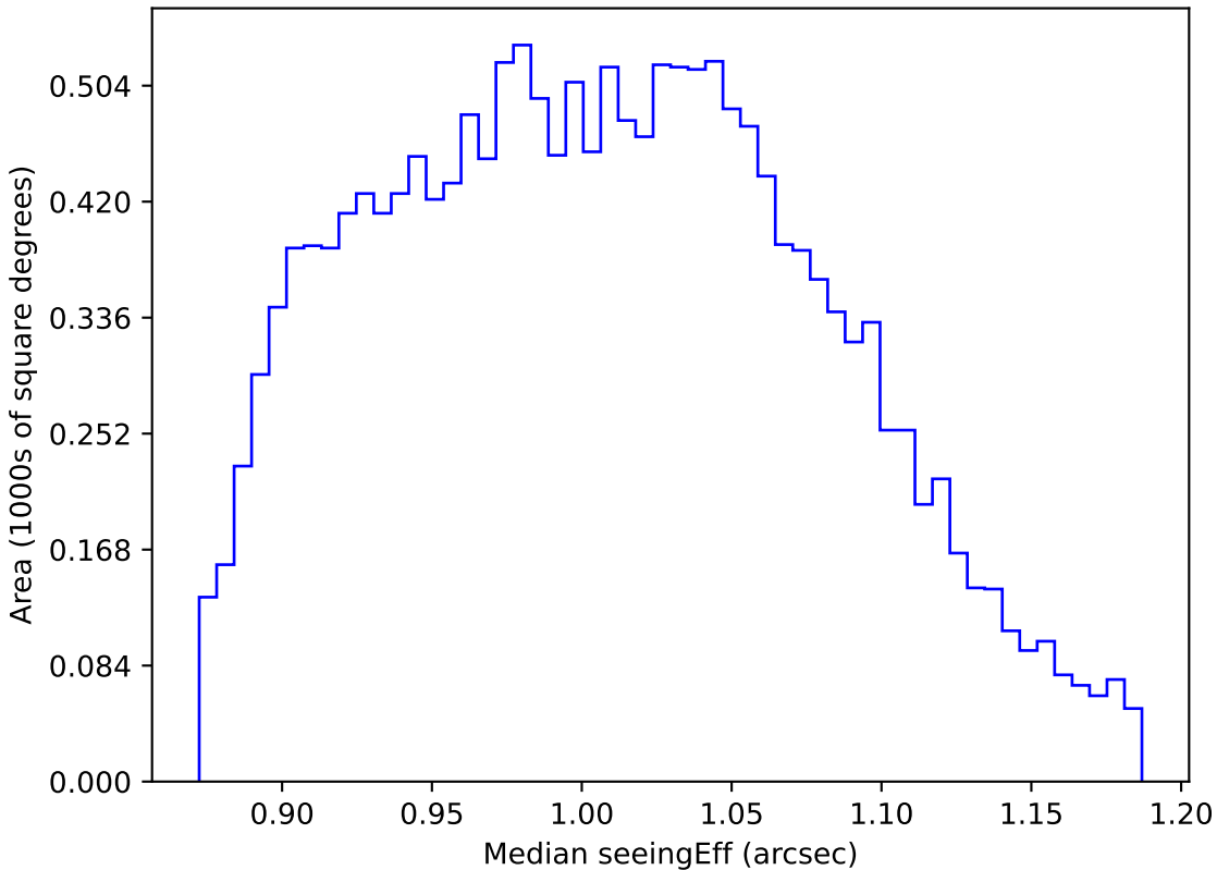
baseline_v3.3_10yrs WFD z band: Median seeingEff
