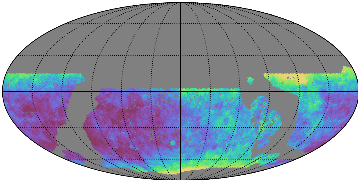
baseline_v3.3_10yrs WFD y band: Median seeingEff
