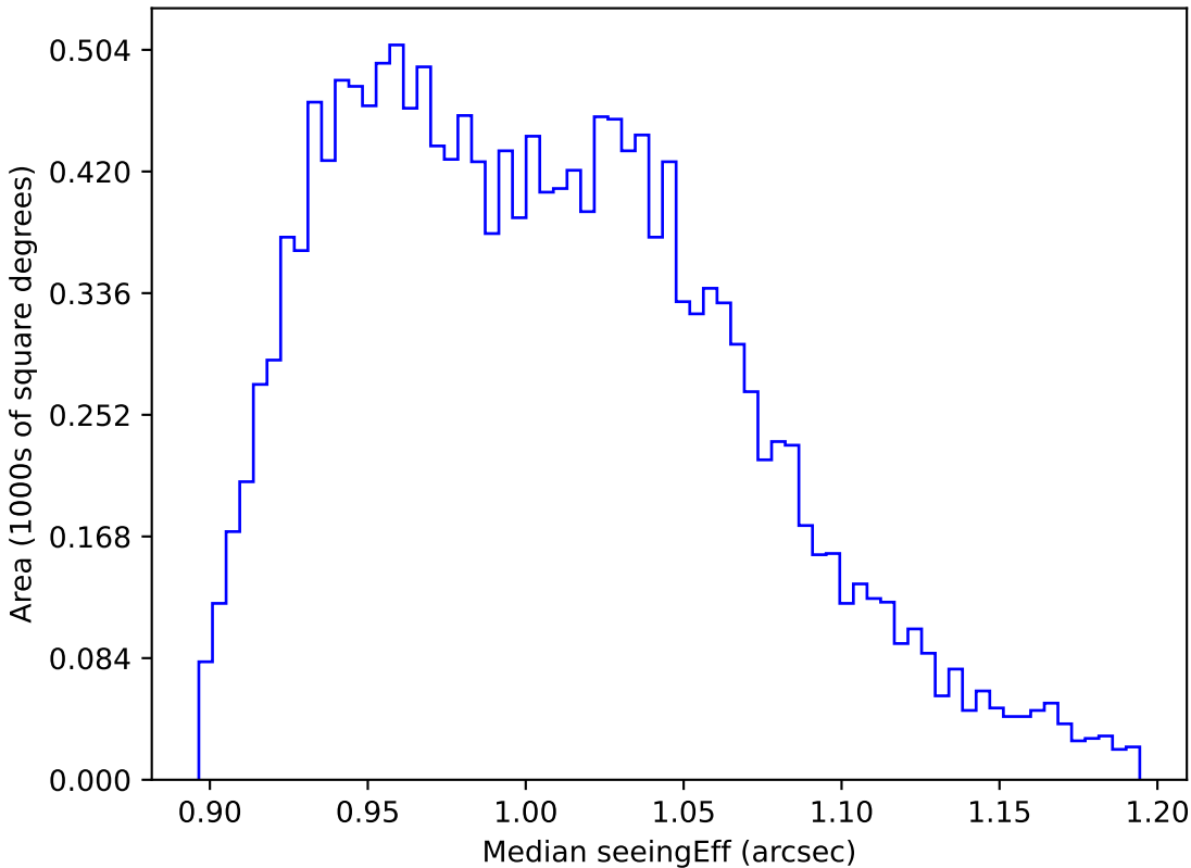
baseline_v3.3_10yrs WFD y band: Median seeingEff
