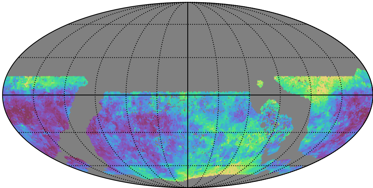
baseline_v3.3_10yrs WFD u band: Median seeingEff
