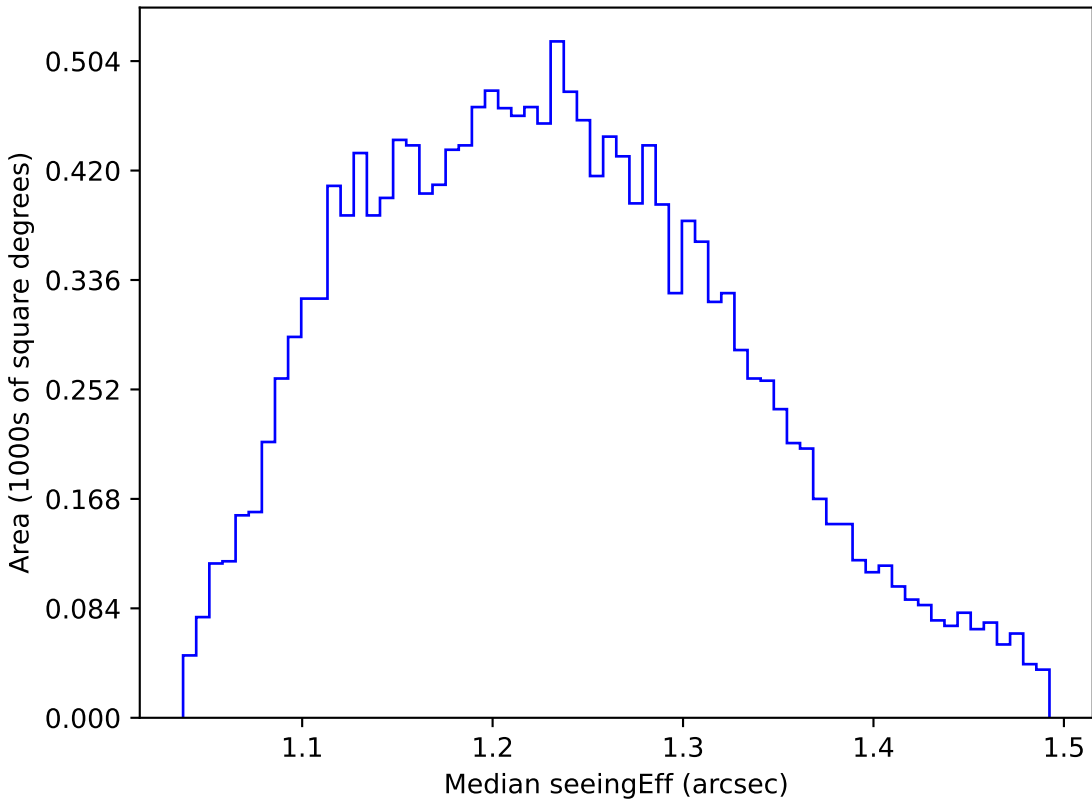
baseline_v3.3_10yrs WFD u band: Median seeingEff
