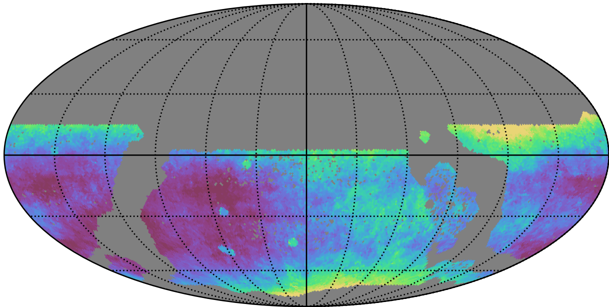
baseline_v3.3_10yrs WFD r band: Median seeingEff
