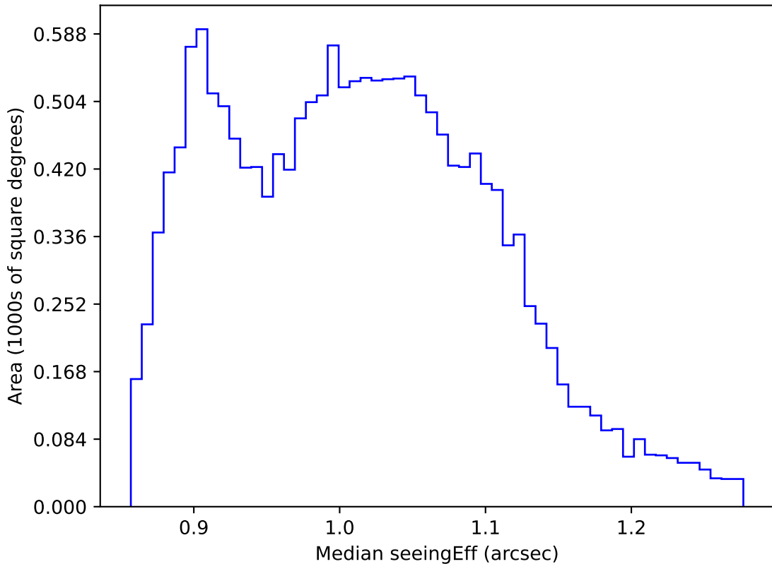
baseline_v3.3_10yrs WFD r band: Median seeingEff
