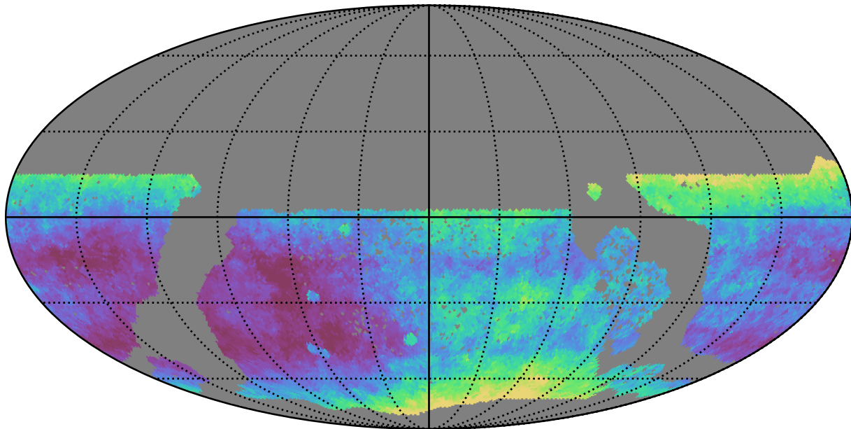
baseline_v3.3_10yrs WFD i band: Median seeingEff
