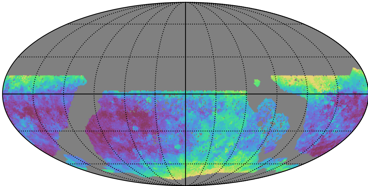
baseline_v3.3_10yrs WFD g band: Median seeingEff
