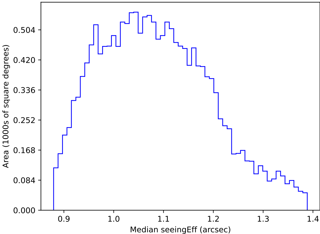
baseline_v3.3_10yrs WFD g band: Median seeingEff
