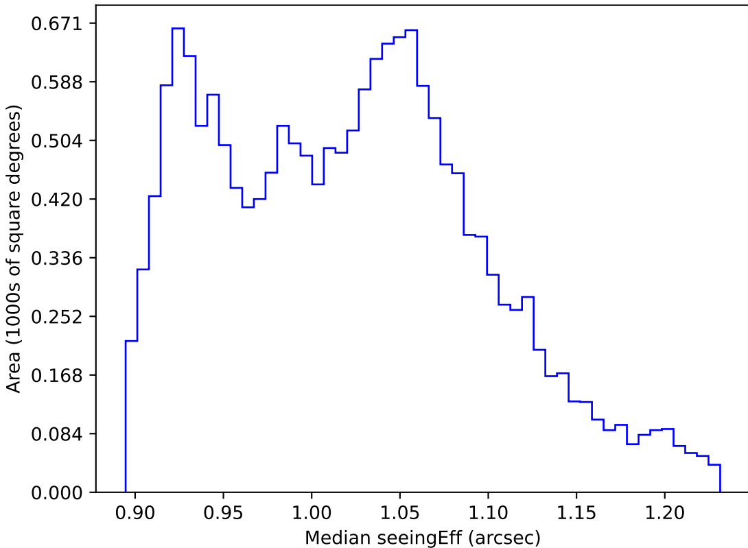
baseline_v3.3_10yrs WFD all bands: Median seeingEff
