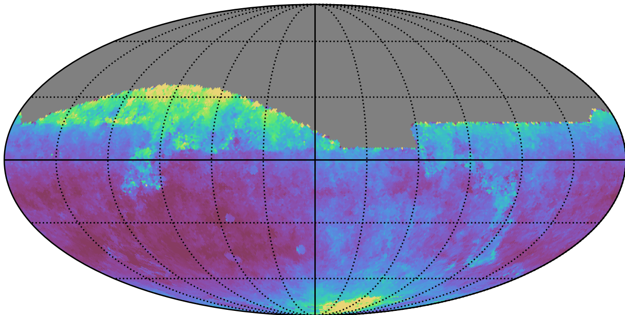
baseline_v3.3_10yrs All sky z band: Median seeingEff
