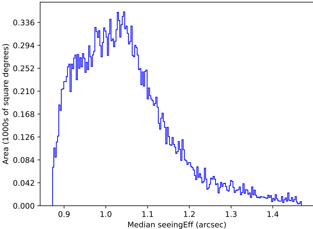
baseline_v3.3_10yrs All sky z band: Median seeingEff
